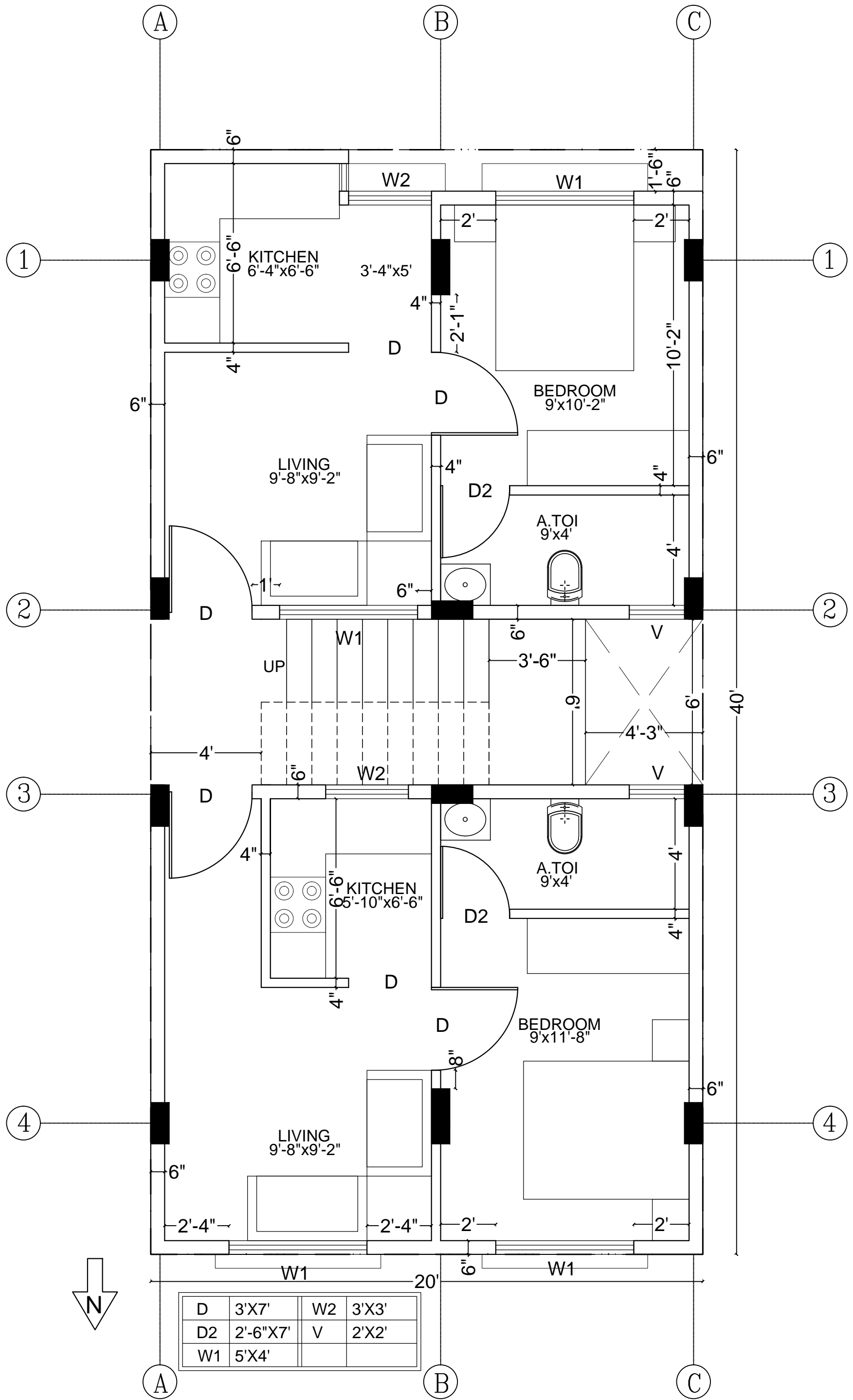
TYPICAL FLOOR PLAN 1 , 2 & 3
